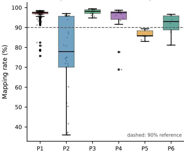
Mapping rate by panel (P2 suffers reference bias)
