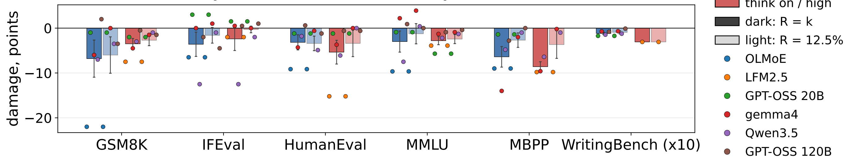
Per benchmark (bars: mean over models)
