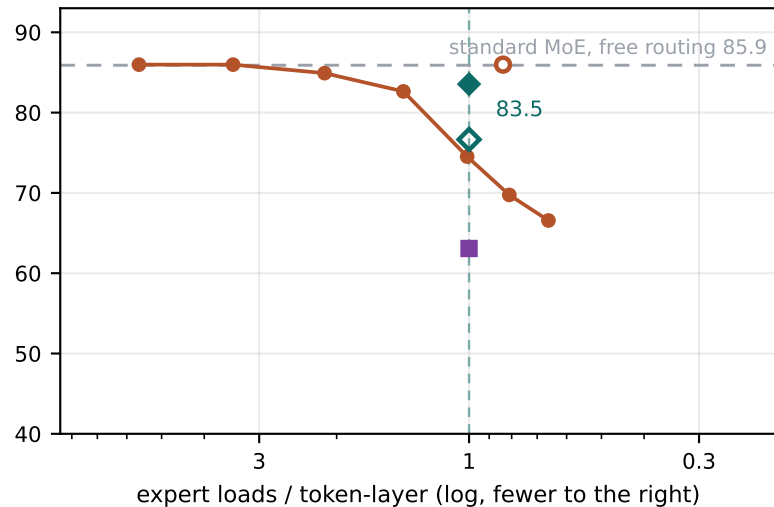
Qwen3.5, 32x memory reduction
