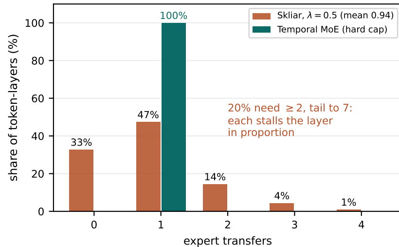
transfers in one token-layer (gemma4)
