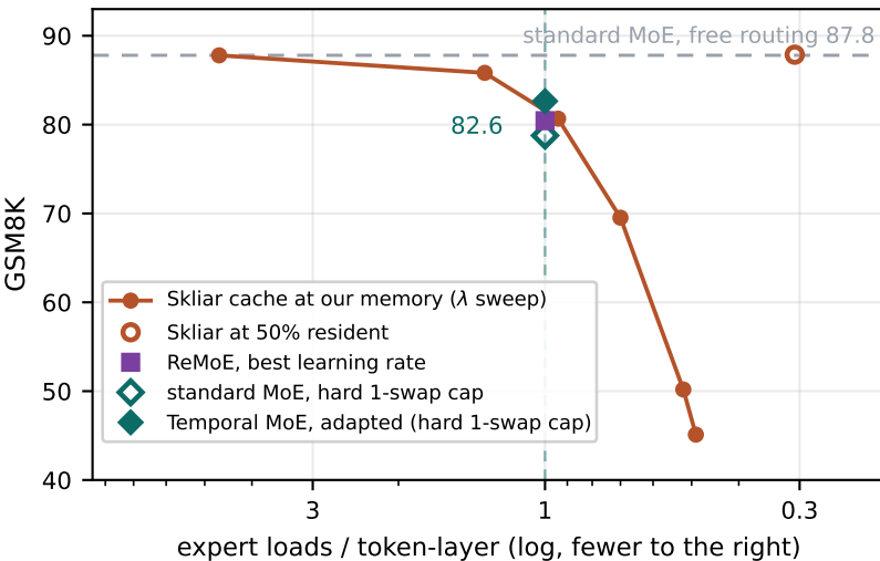
gemma4, 16x memory reduction
