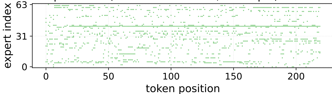
Temporal MoE (constraint removed, free top-k)
