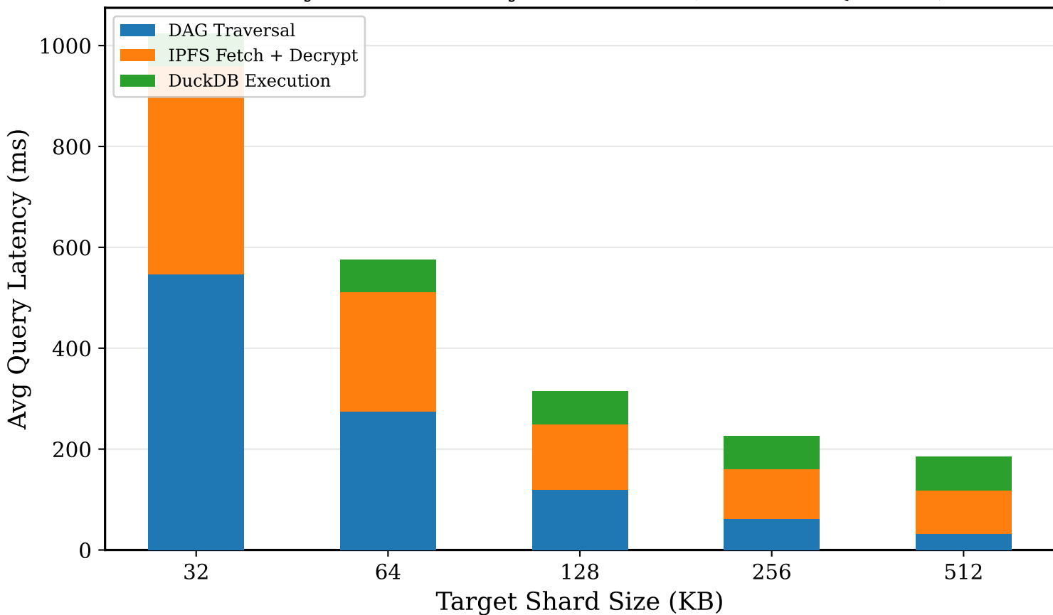
Latency Breakdown by Shard Size (Selective Queries)
