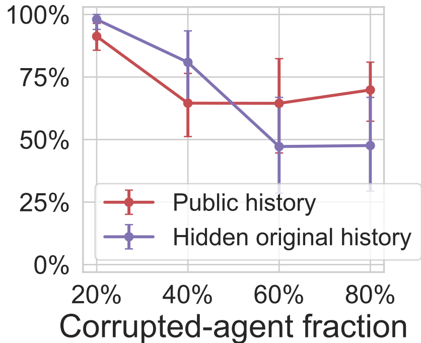
Honest-action match rate
