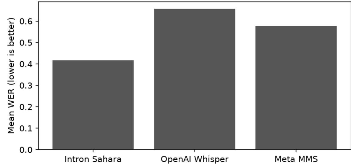
Domain 1: Overall WER by model
