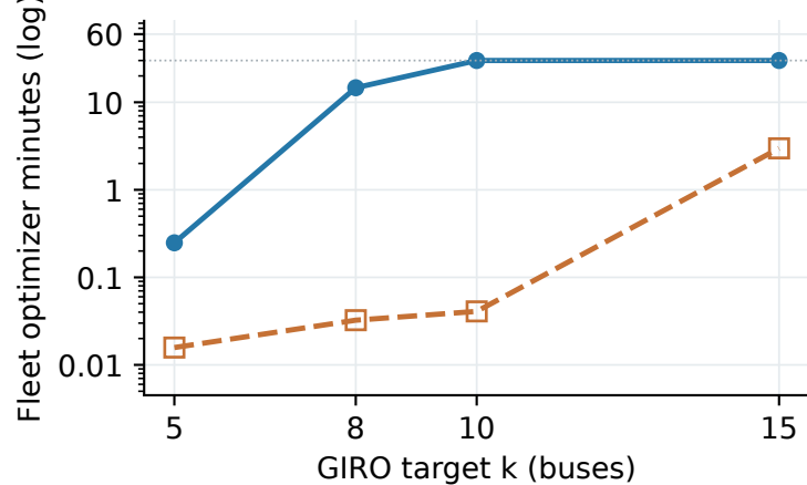
MIP: fleet search
