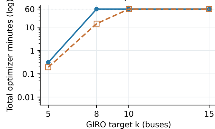
MIP: total optimizer time
