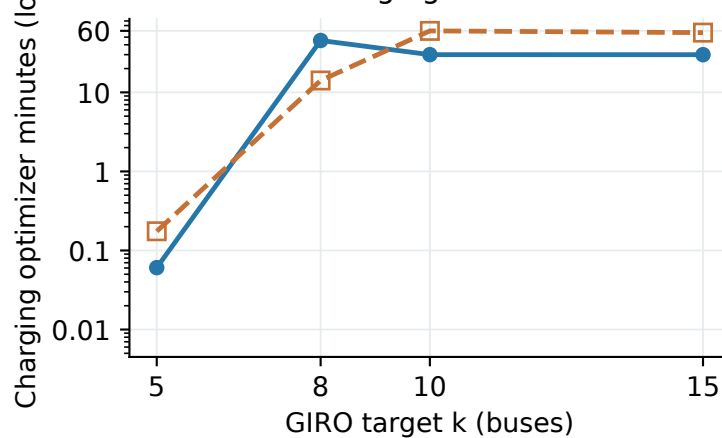
MIP: charging-cost search
