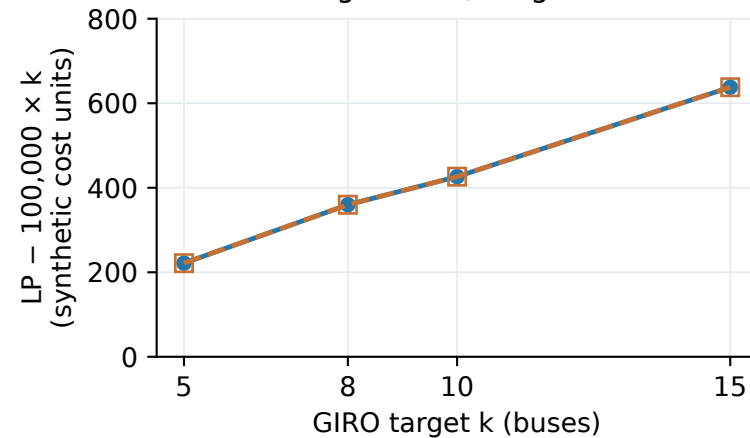
Weighted LP, magnified
