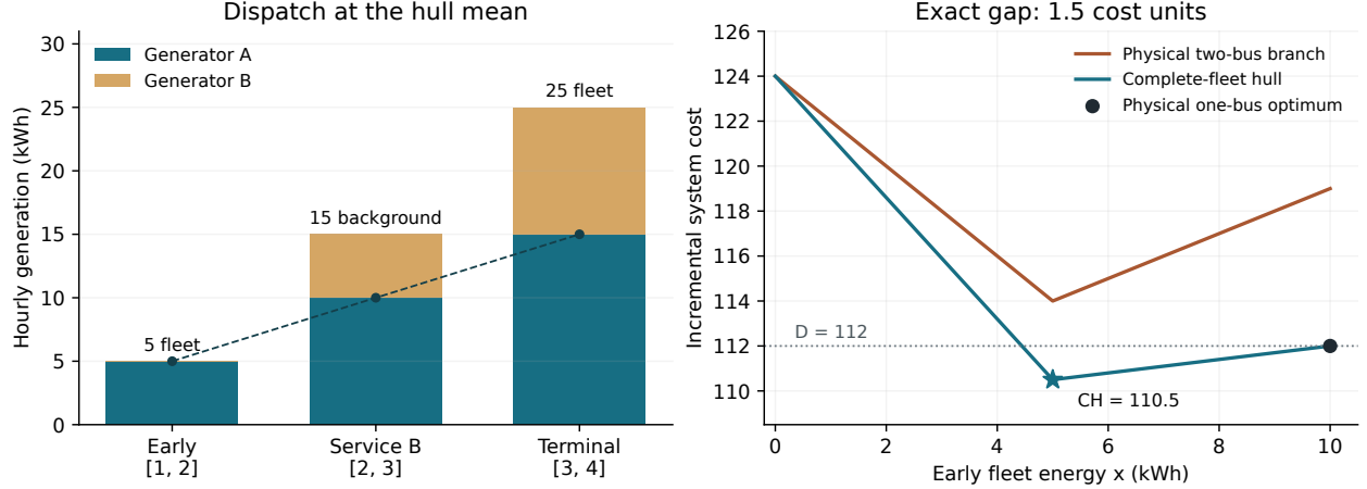
Figure 5: The hourly generation example. Left: generation serving the hull mean; the middle hour serves only background demand, and A rises by its 5-unit limit in each interval. Right: physical two-bus and hull costs over the full continuous charging interval, with the one-bus optimum marked separately. All costs and offers are synthetic.
