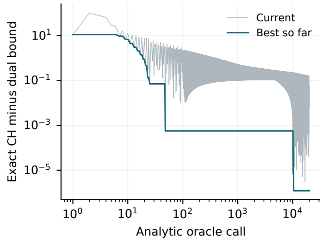
Different dual diagnostics
