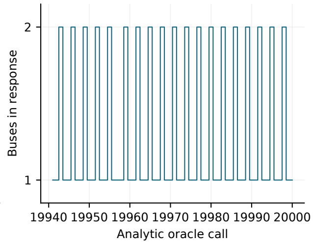
Switching persists in this run
