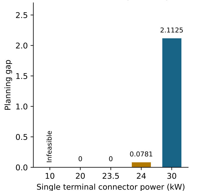
(b) Reserve 0; efficiency 1; early 10 kW
