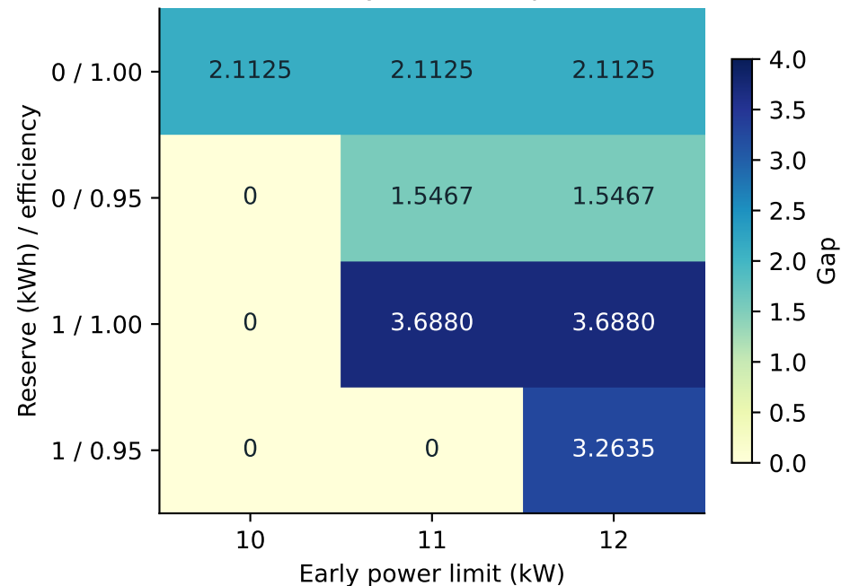
(a) Fixed battery; terminal power 30 kW
