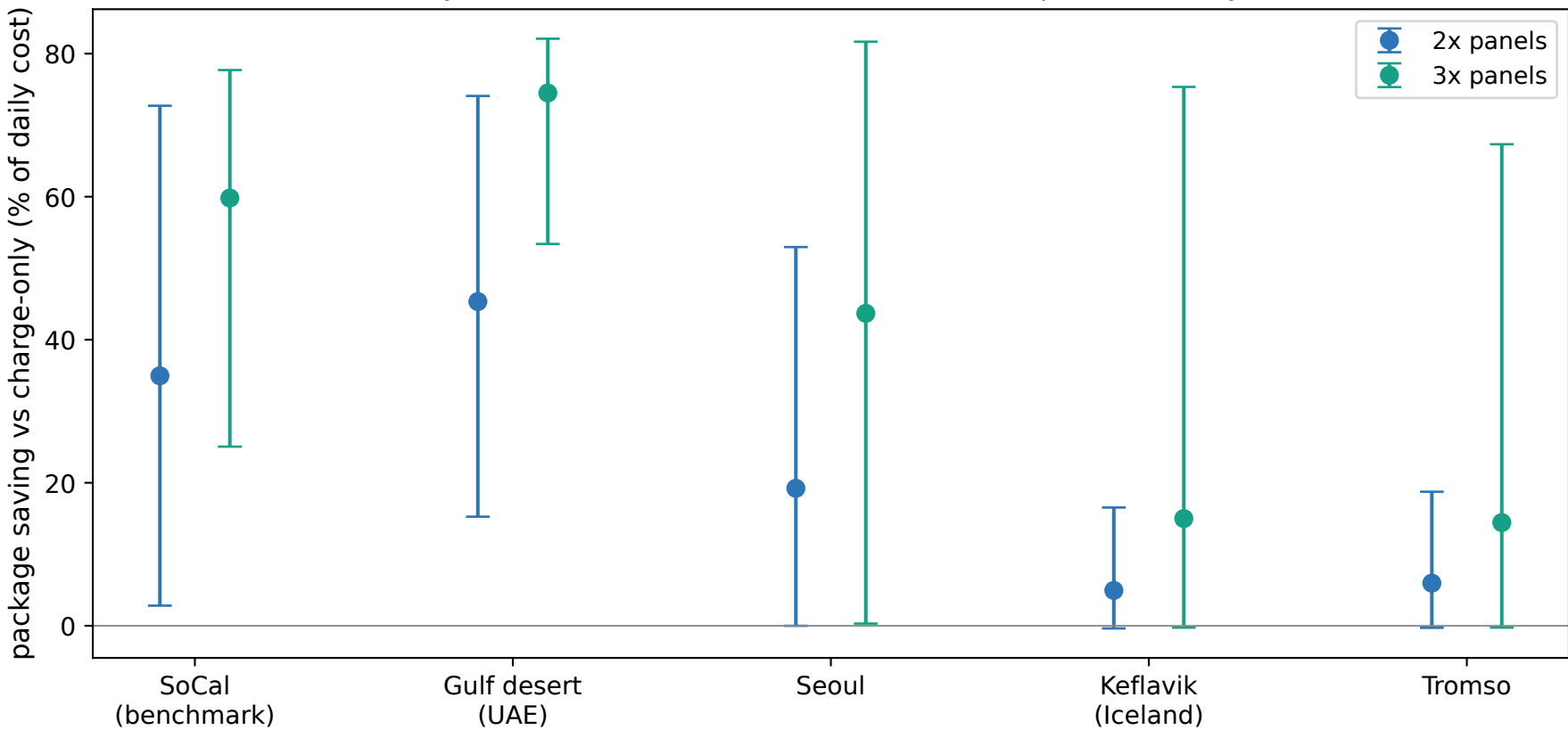
same array, five skies: annual mean and 10th-90th percentile days (2023)
