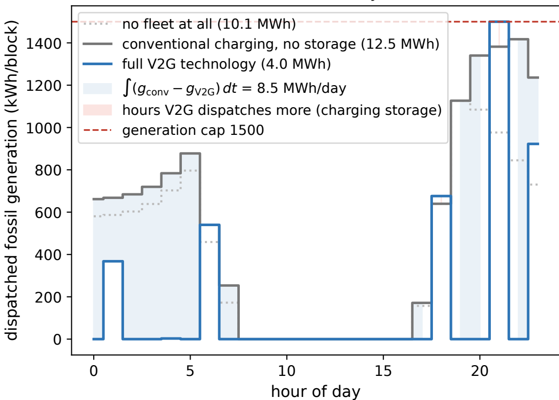
same fleet, same tasks: V2G cuts daily fossil 12.5 -> 4.0 MWh
