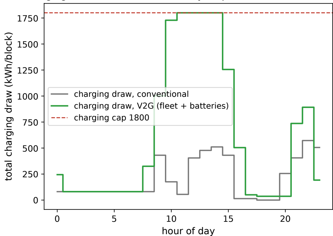
charging concentrates in the midday surplus, under the station
