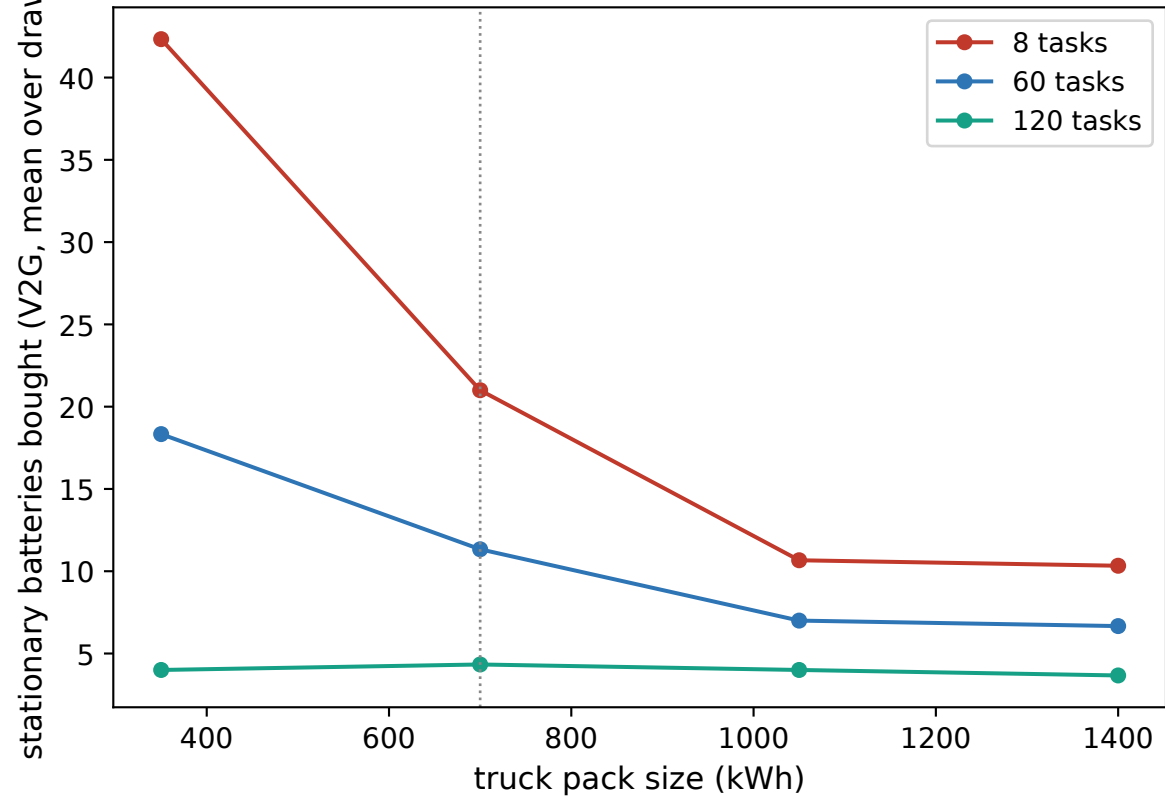
pack x workload: the substitution at 8-120 tasks (2x solar)
