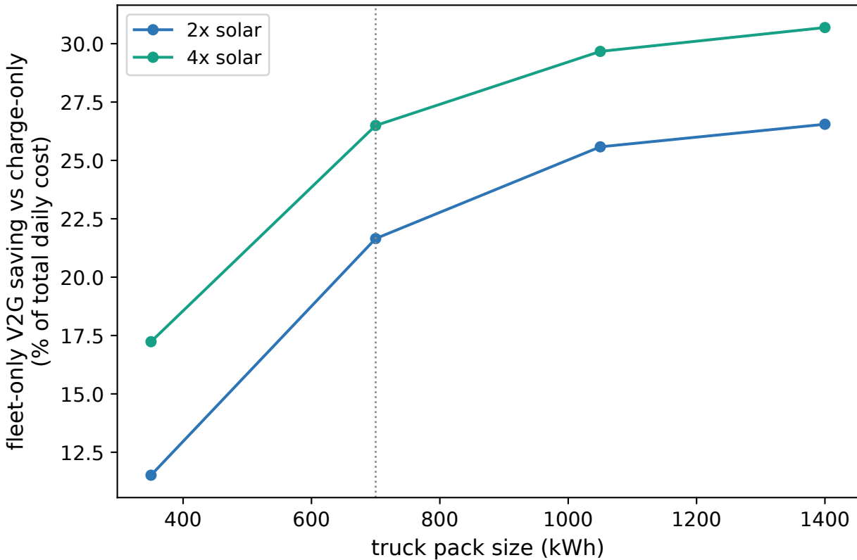
bigger packs raise fleet-as-storage value, with saturation
