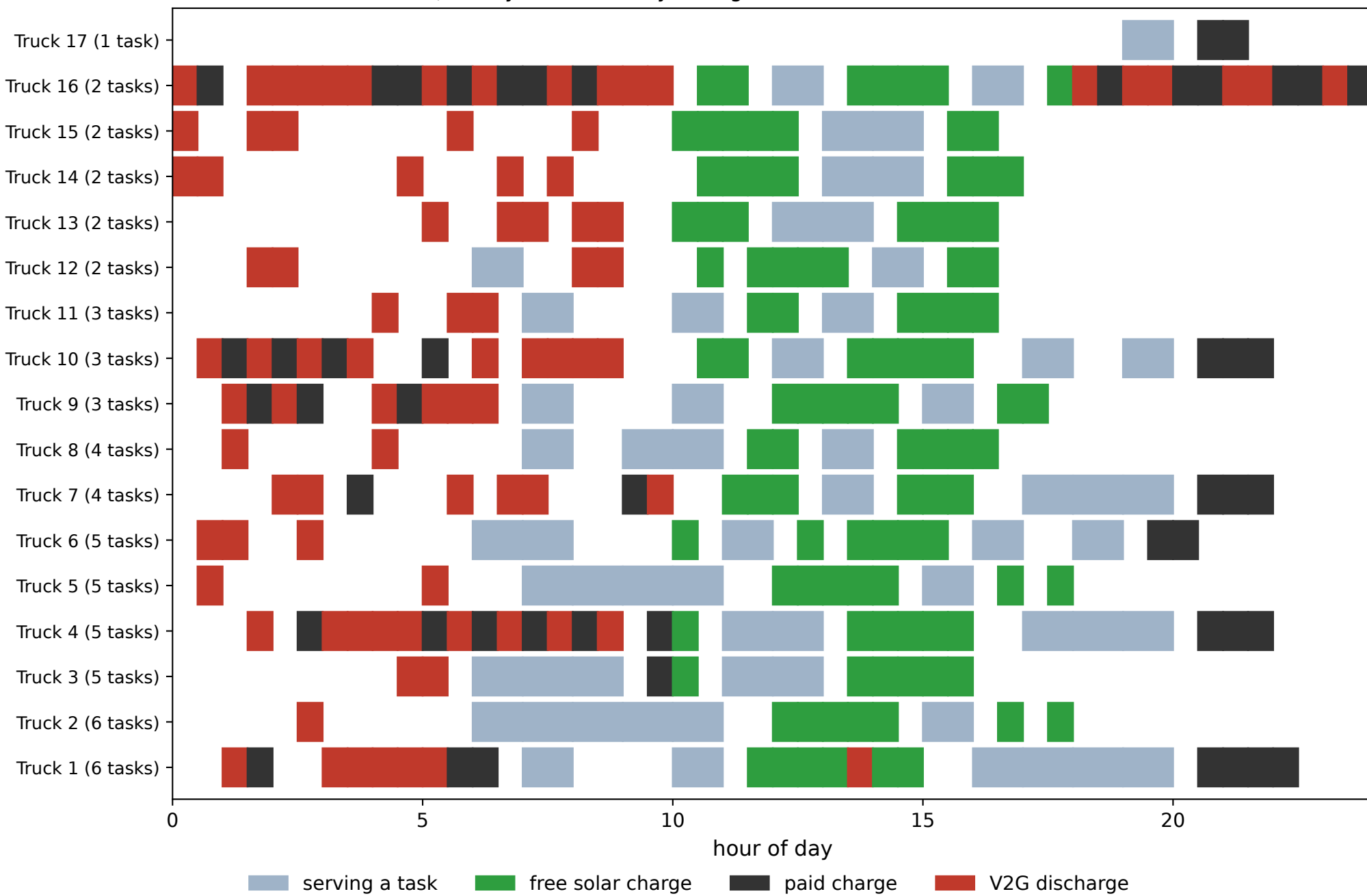
truck $45/day, no stationary storage: 17 trucks (3.5 tasks/truck), 0 batteries
