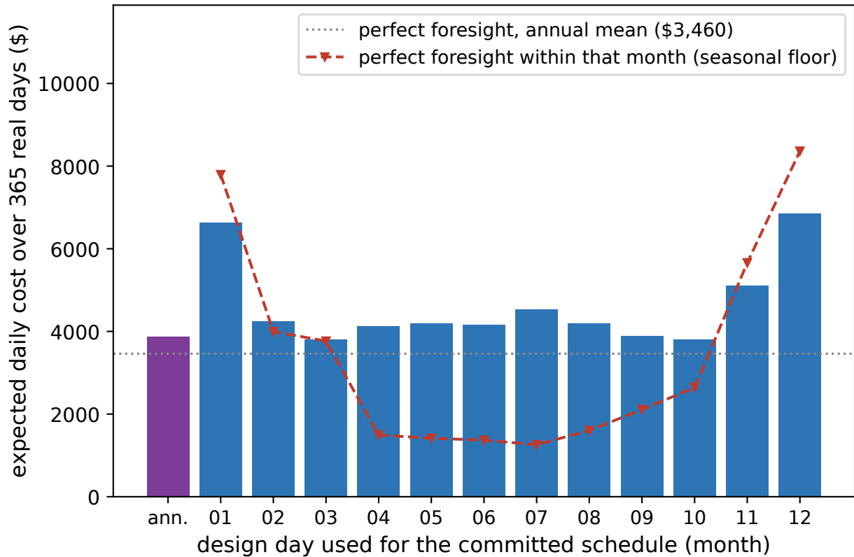
(b) 3x panels: best commit +9.7% vs clairvoyance
