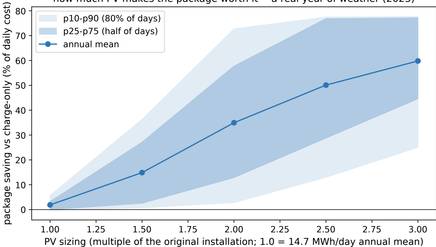
how much PV makes the package worth it -- a real year of weather (2023)
