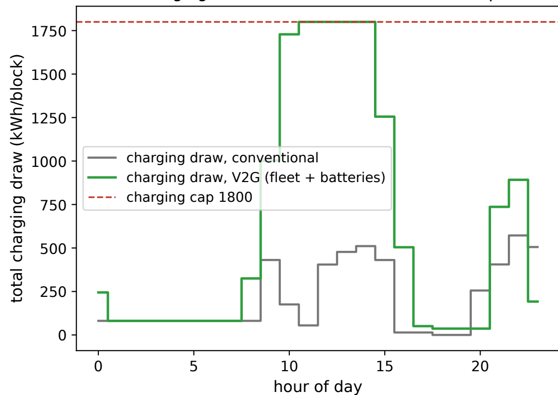
charging concentrates under the station cap
