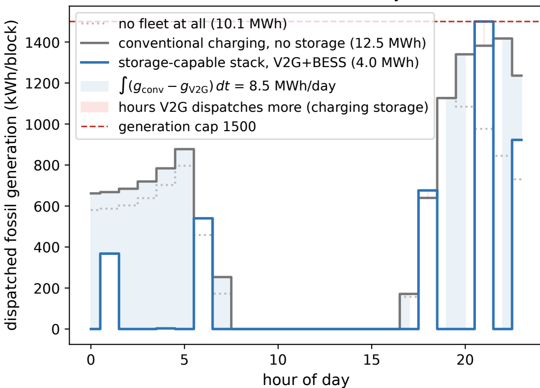
same fleet, same tasks: the full stack cuts daily fossil 12.5 -> 4.0 MWh
