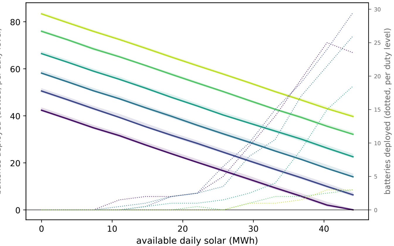
(b) 150 tasks: heavy duties never reach zero
