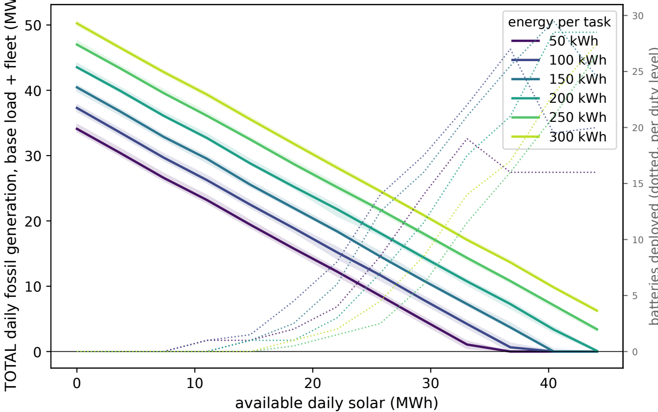
(a) 60 tasks: enough solar zeroes out ALL generation
