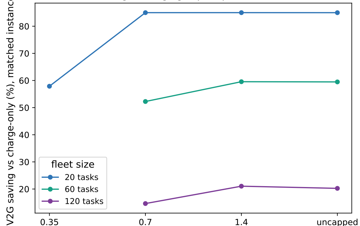
(b) tight charging caps clip V2G's value
