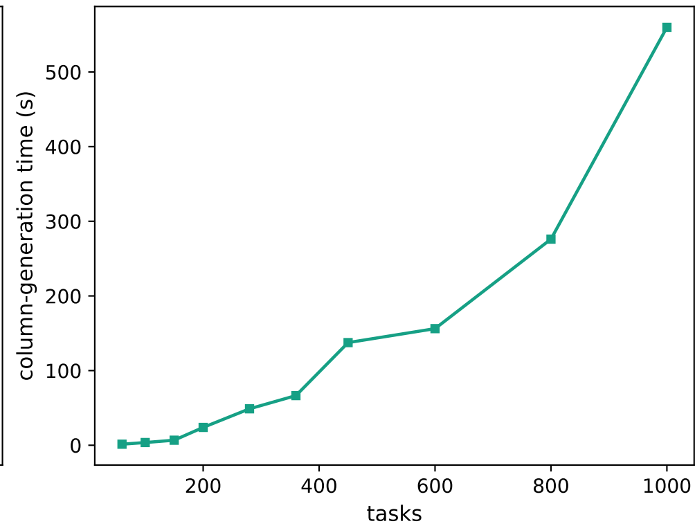
random fleets, multi-station model (cluster)
