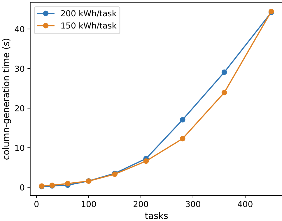
benchmark family (laptop)
