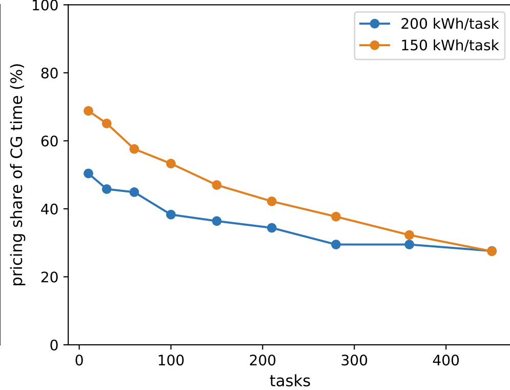
where the time goes
