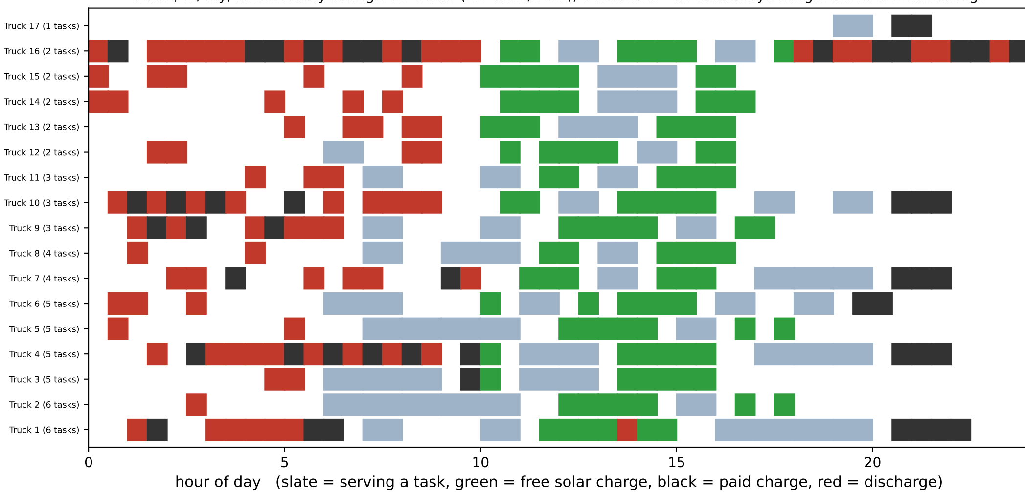
truck $45/day, no stationary storage: 17 trucks (3.5 tasks/truck), 0 batteries -- no stationary storage: the fleet is the storage
