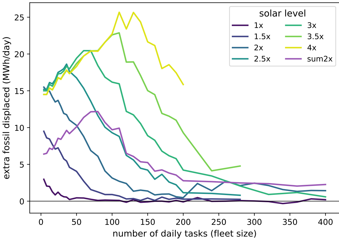
the V2G advantage: grows with sun, fades with fleet size
