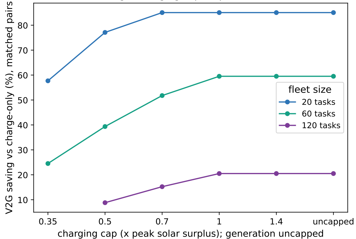
(b) tight charging caps clip V2G's value
