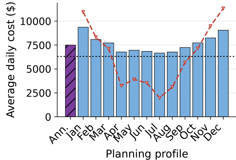
(a) 2x solar
