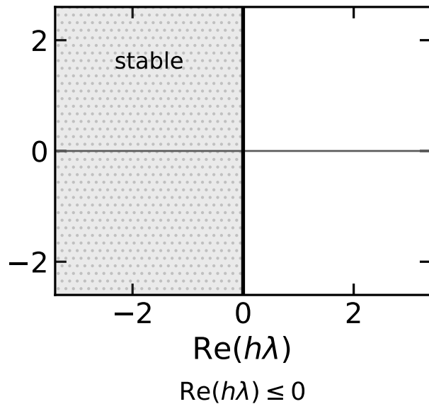
trapezoid (Crank-Nicolson) A-stable
