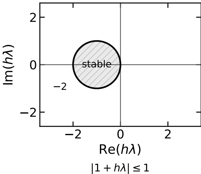
forward Euler not A-stable
