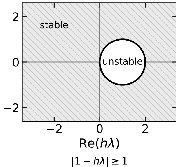
backward Euler A-stable
