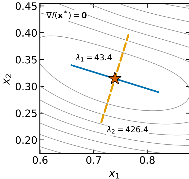
zoomed on \mathbf{x}^*
