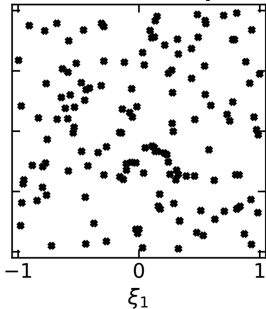
Nested sparse grid (145 points) Monte Carlo (145 points)
