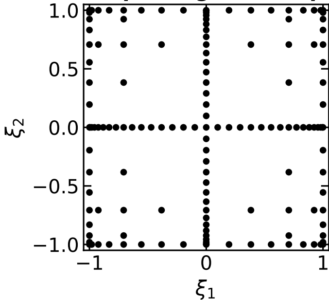
Nested sparse grid (145 points) Monte Carlo (145 points)
