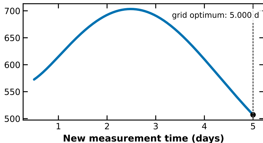
ME: minimize condition number
