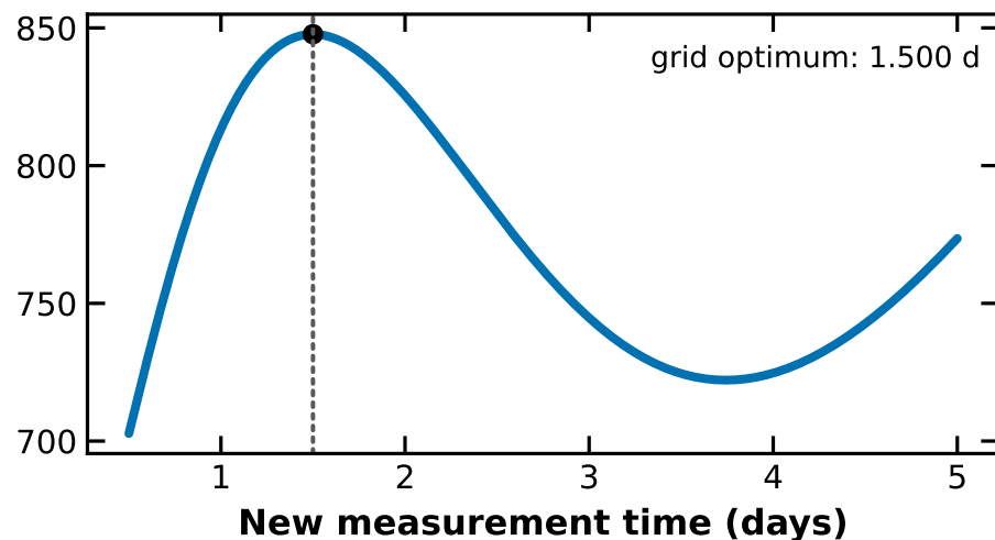
D: maximize determinant
