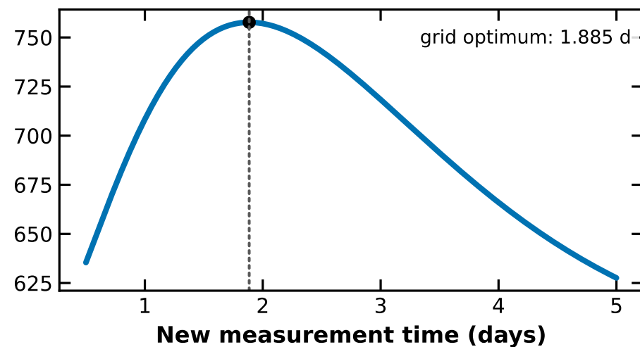
Pseudo-A: maximize trace
