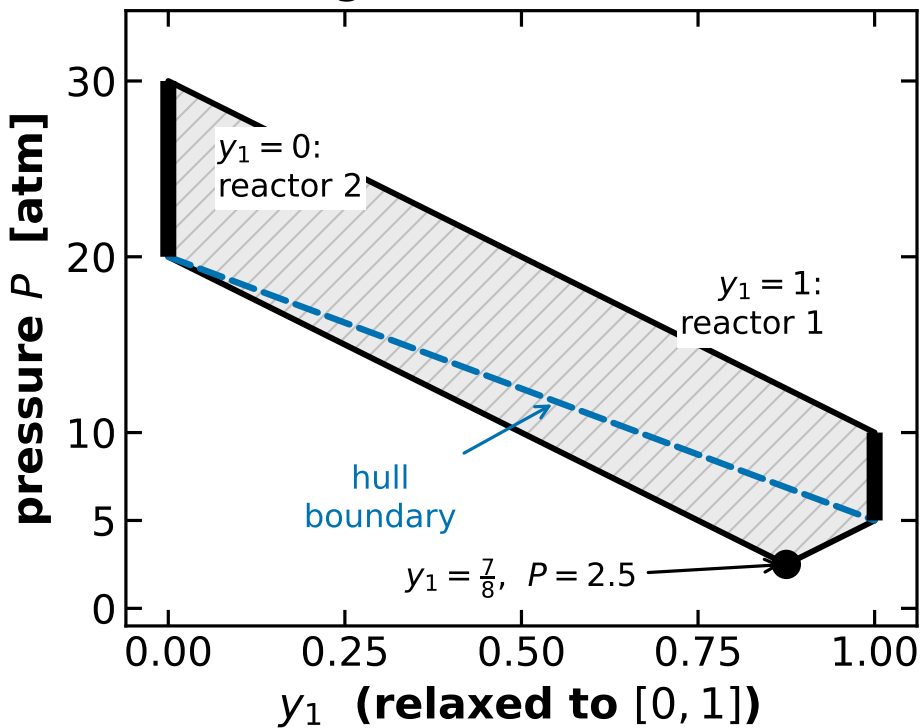
big- M ( M_1 = M_2 = 20 )
