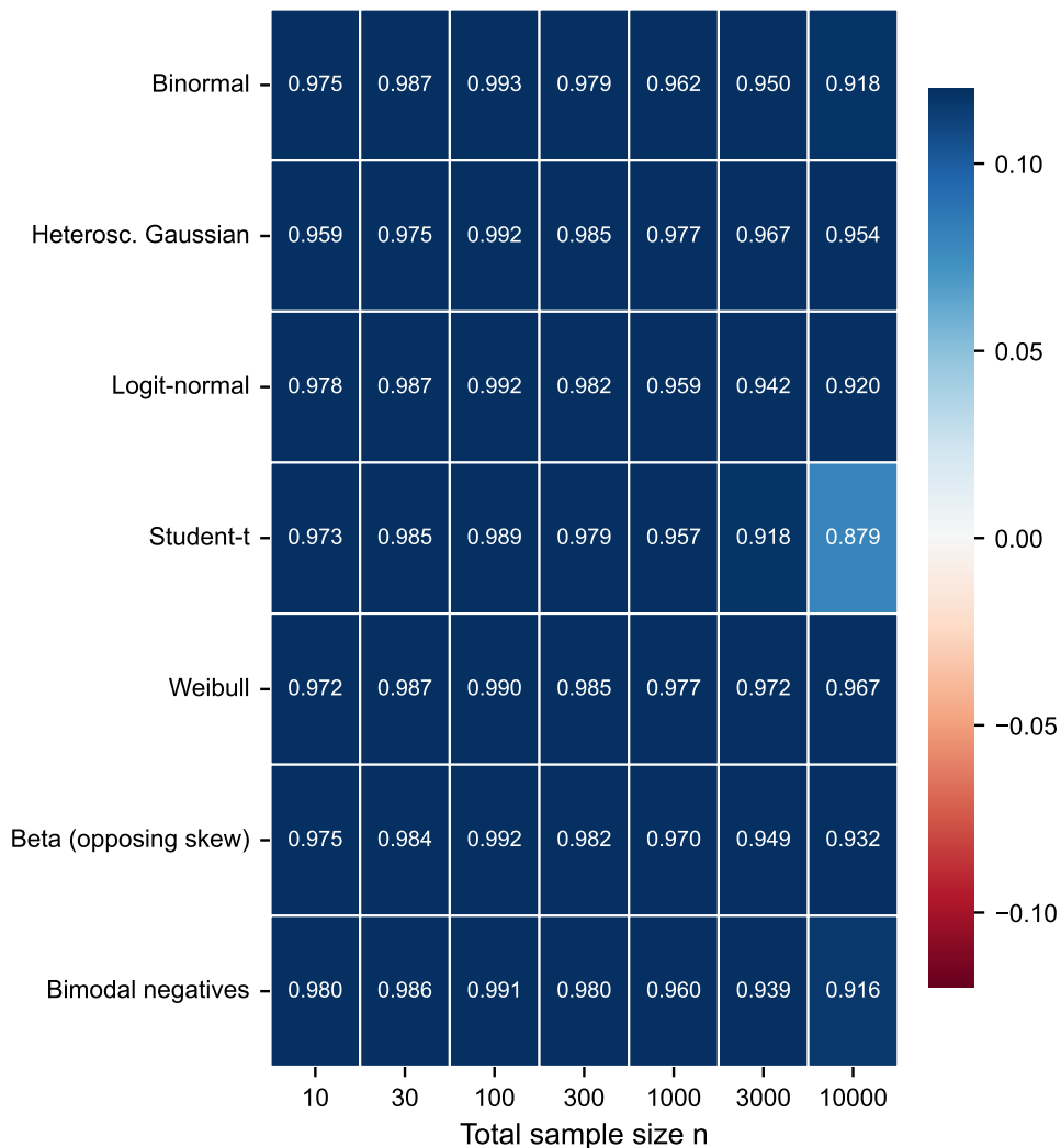
80% band (nominal 0.80)
