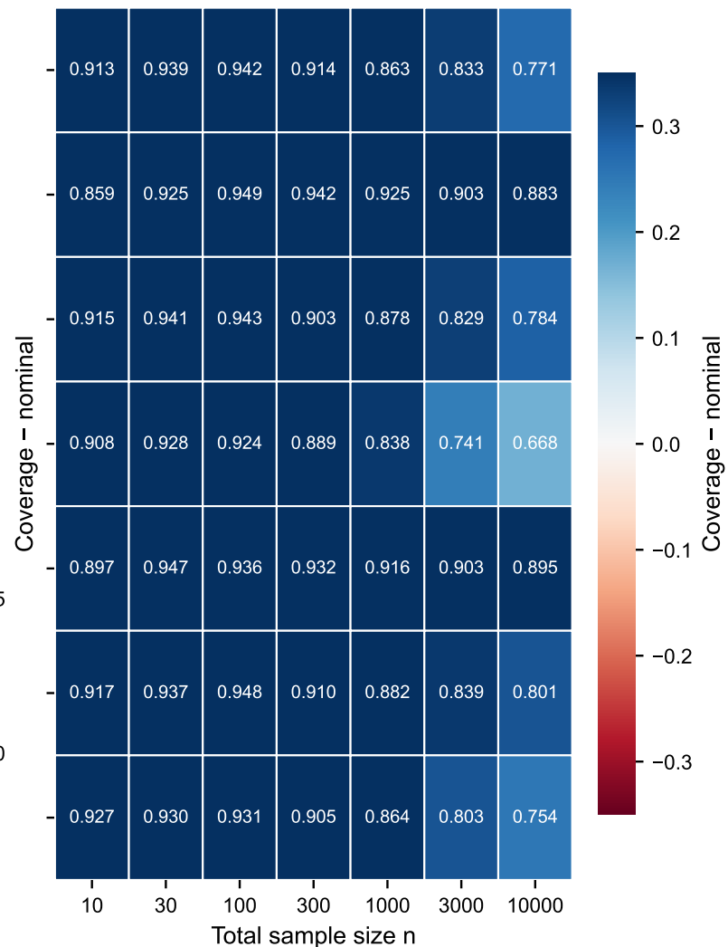
50% band (nominal 0.50)
