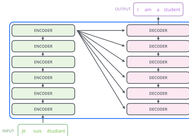
Figure 2: Inter structure of Encoder and Decoder modules
