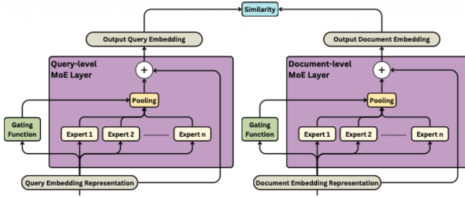
Figure 14: SB-MoE Architecture Overview
