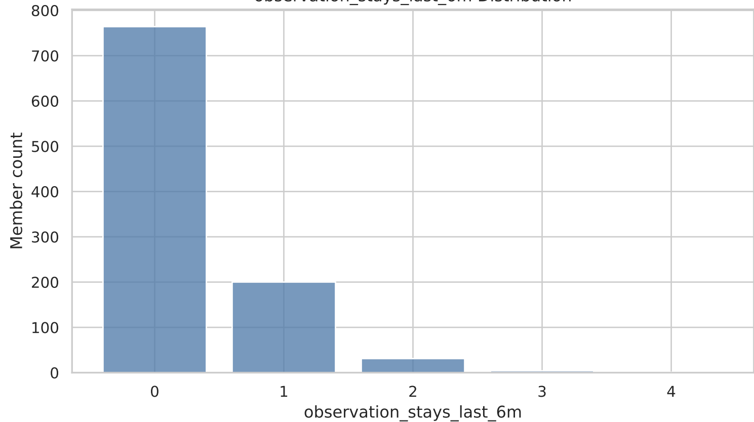
observation_stays_last_6m Distribution
