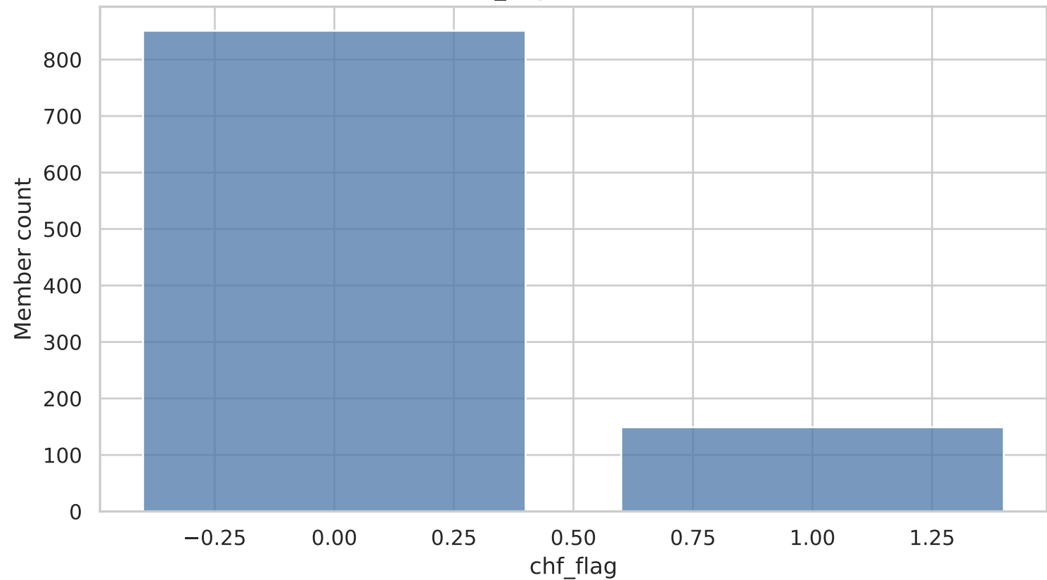
chf_flag Distribution
