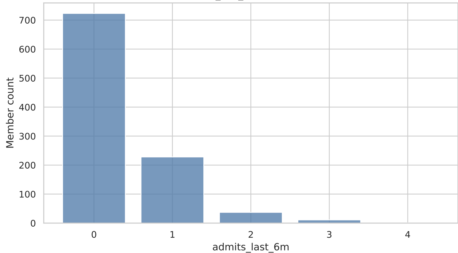
admits_last_6m Distribution
