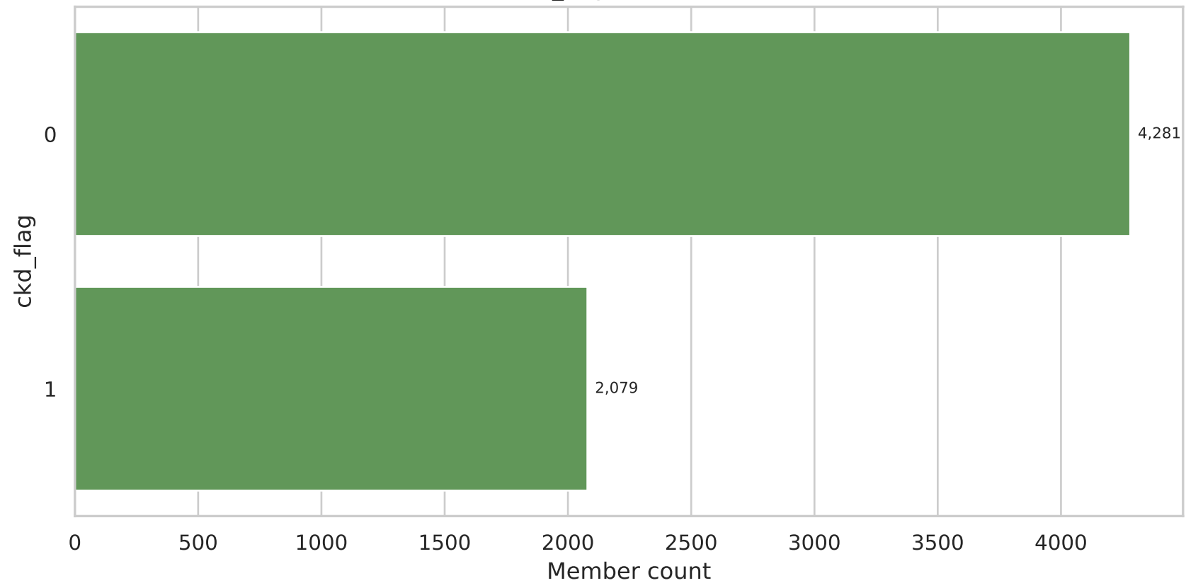
ckd_flag Distribution
