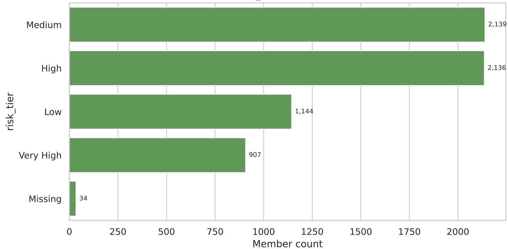
risk_tier Distribution
