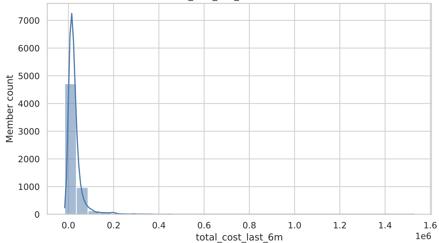
total_cost_last_6m Distribution
