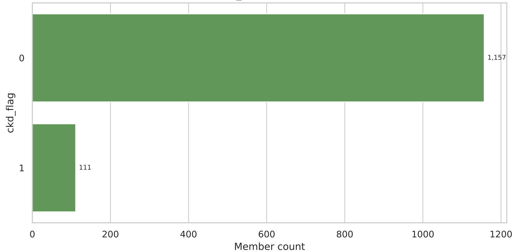
ckd_flag Distribution
