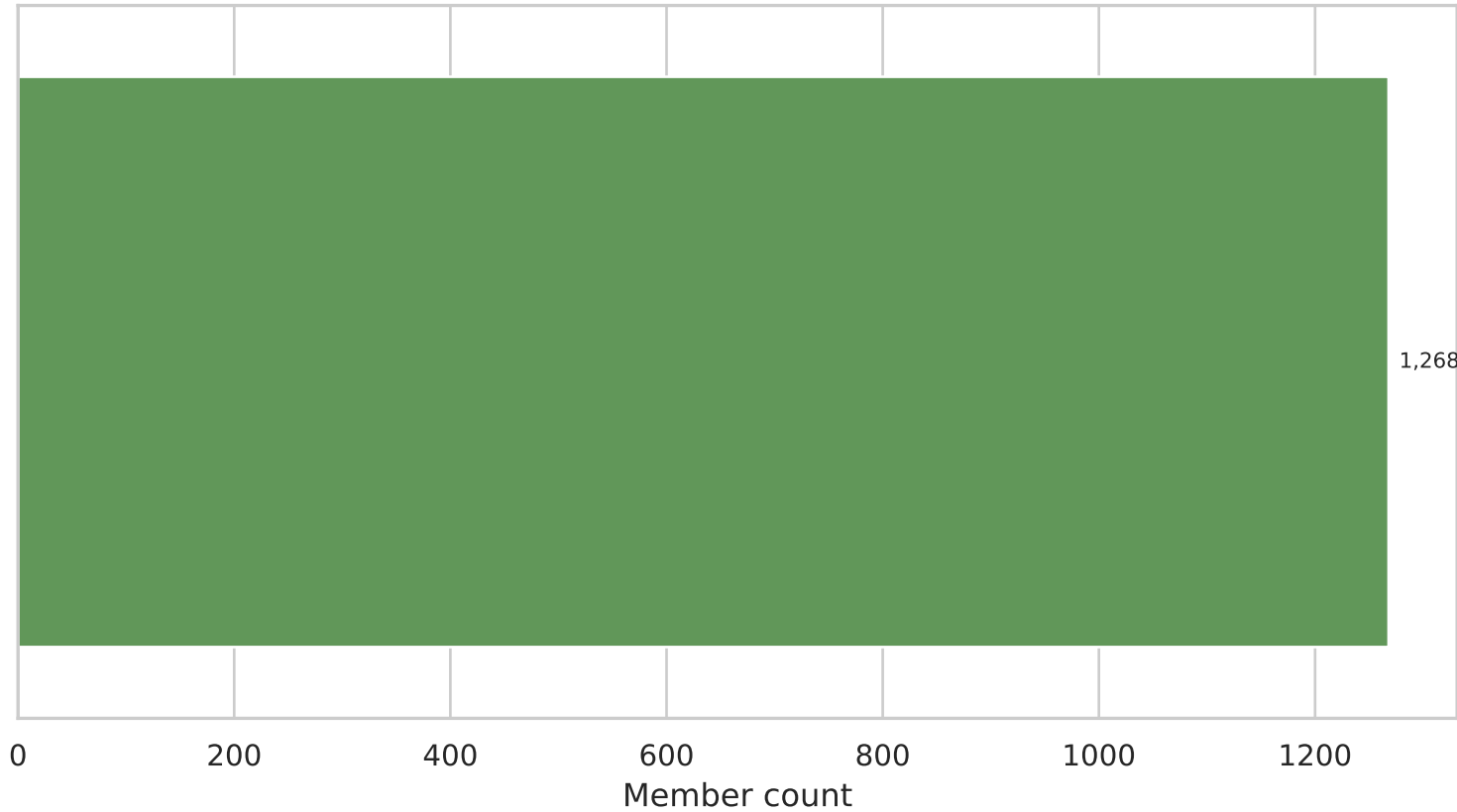
plan_type Distribution
