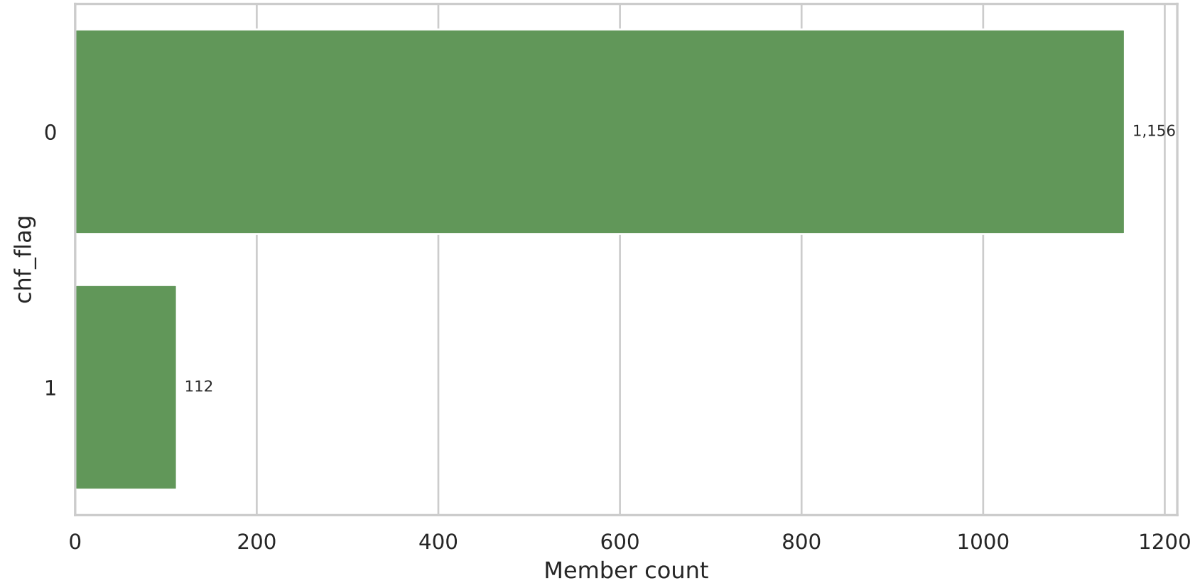
chf_flag Distribution
