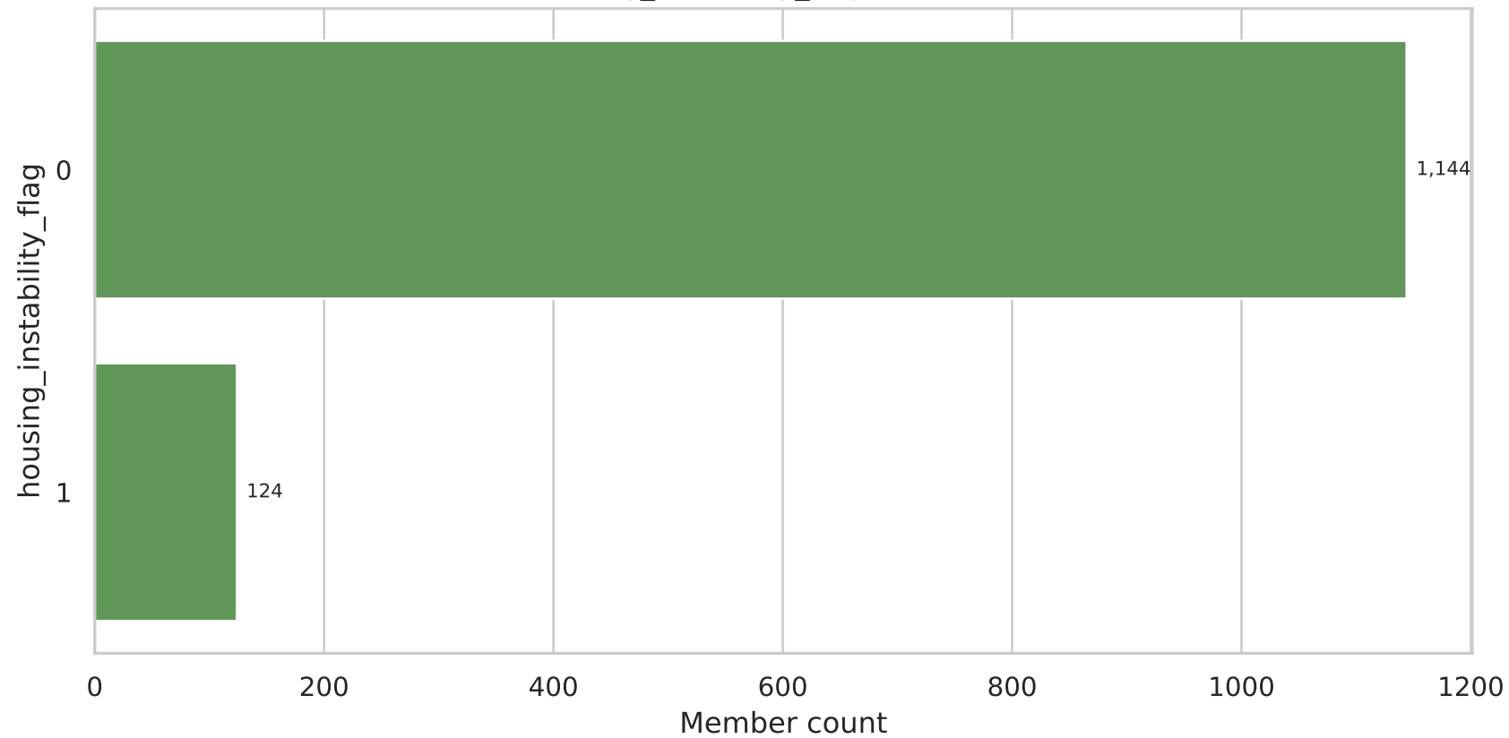
housing_instability_flag Distribution
