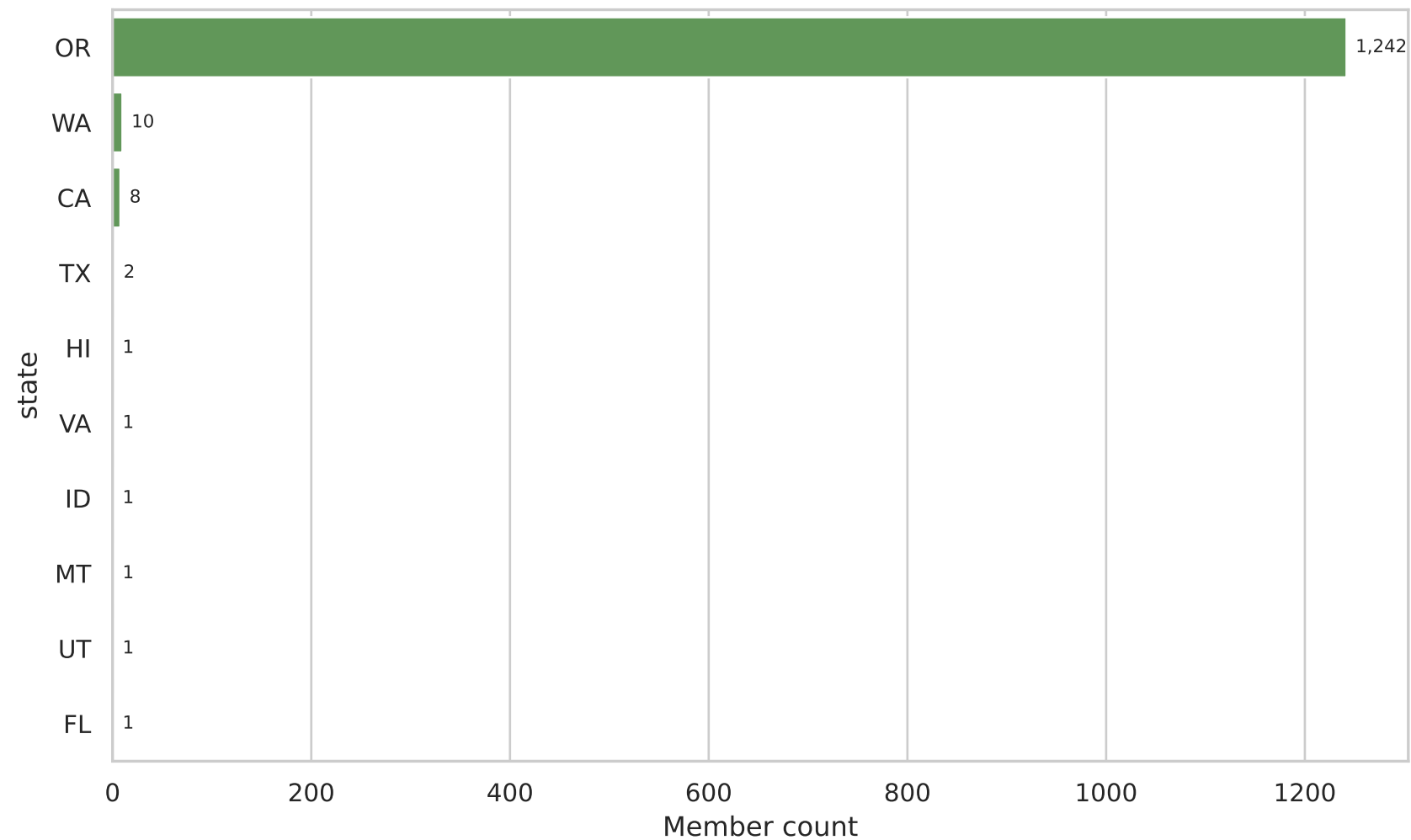
state Distribution
