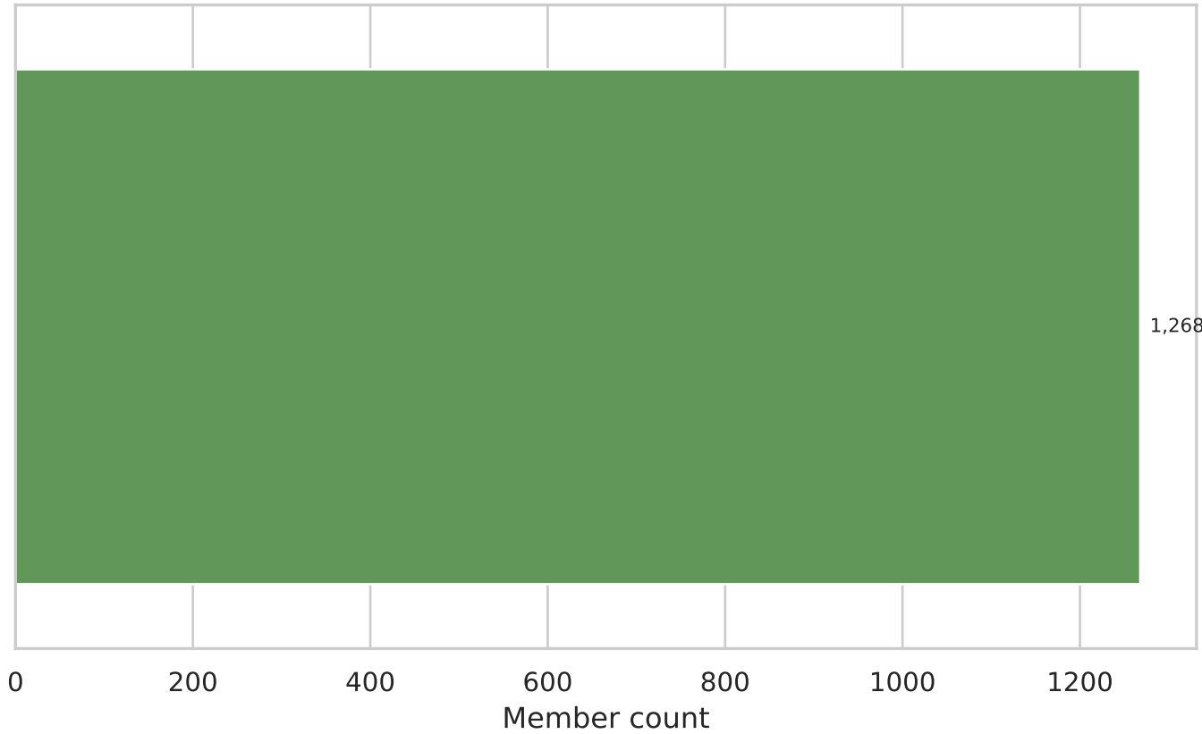
program Distribution
