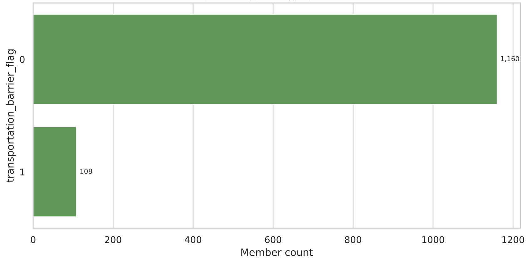
transportation_barrier_flag Distribution
