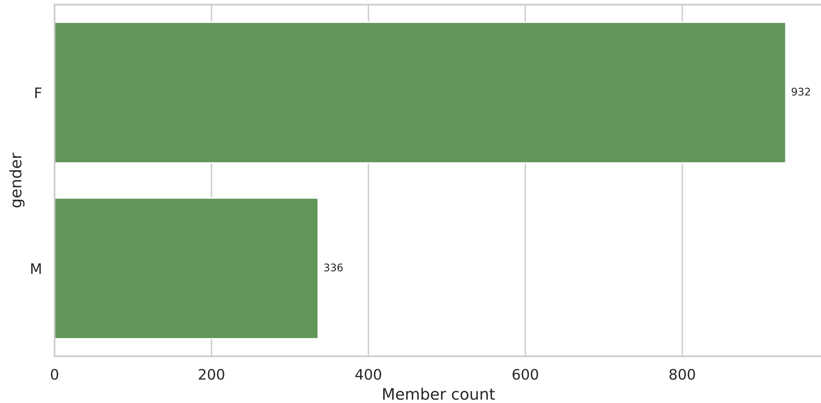
gender Distribution
