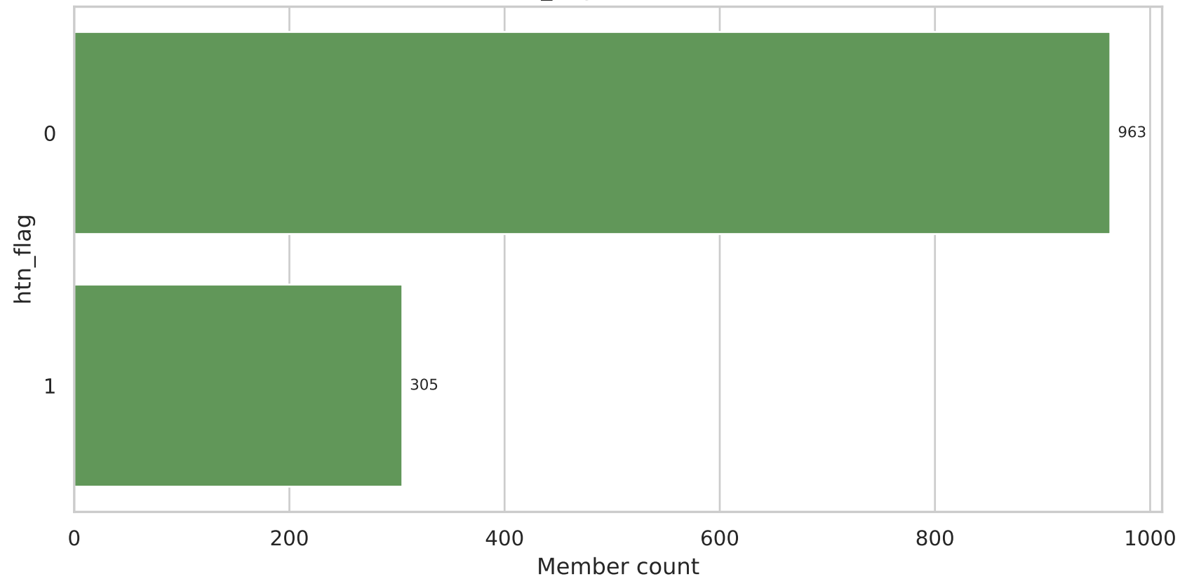
htn_flag Distribution
