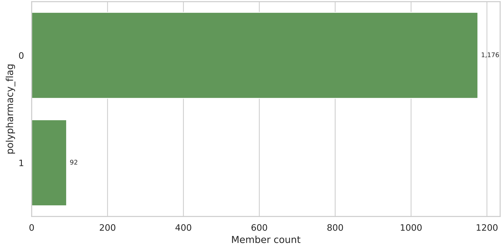
polypharmacy_flag Distribution
