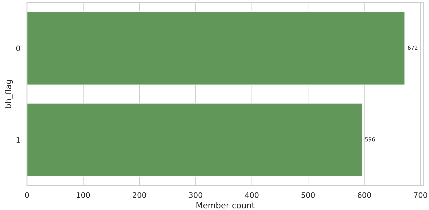
bh_flag Distribution
