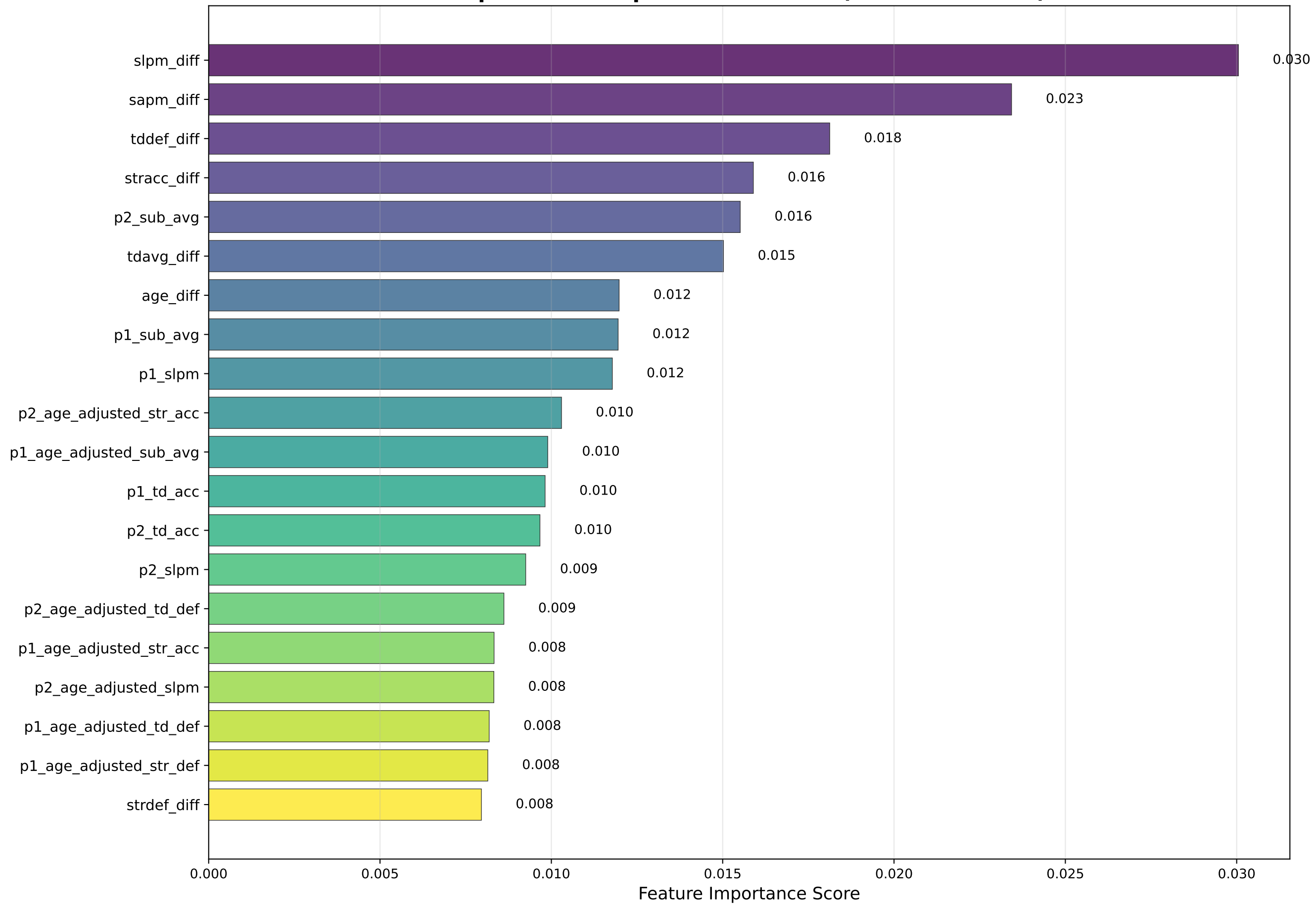
Top 20 Most Important Features (Gradient Colors)
