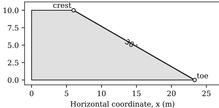
(a) Idealised slope geometry
