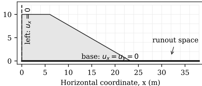
(c) MPM background domain
