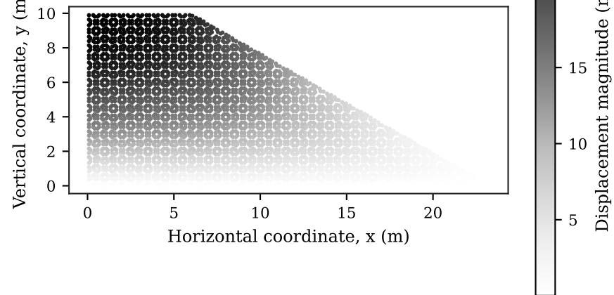
(b) Material-point displacement
