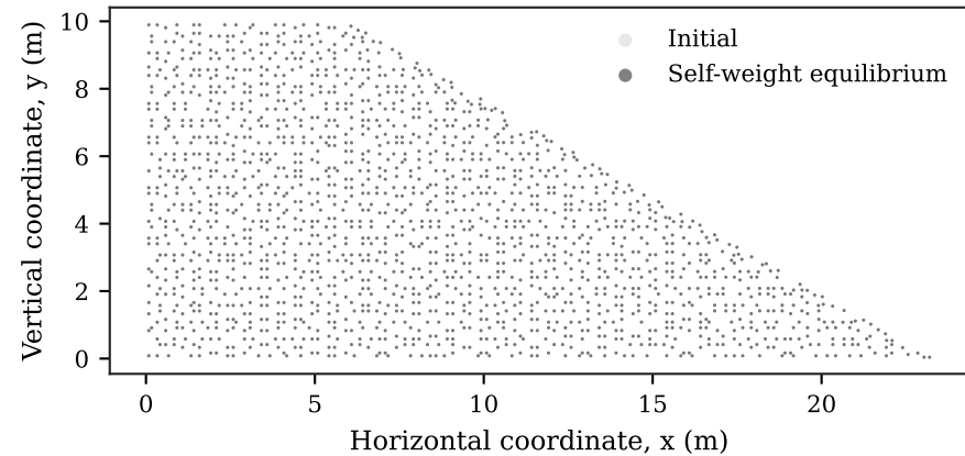
(a) Dry/intact equilibrium configuration
