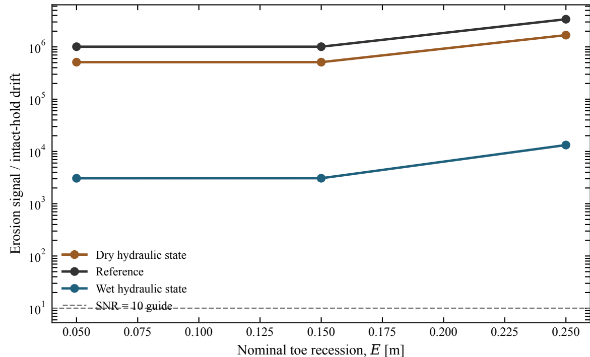
Resolved deformation signal relative to numerical drift
