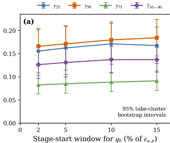
Paired mobilization shift, Stage 2 – Stage 1
