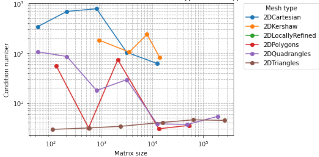
Condition Number vs. Matrix Size for Each Mesh Type in "2D" Type List
