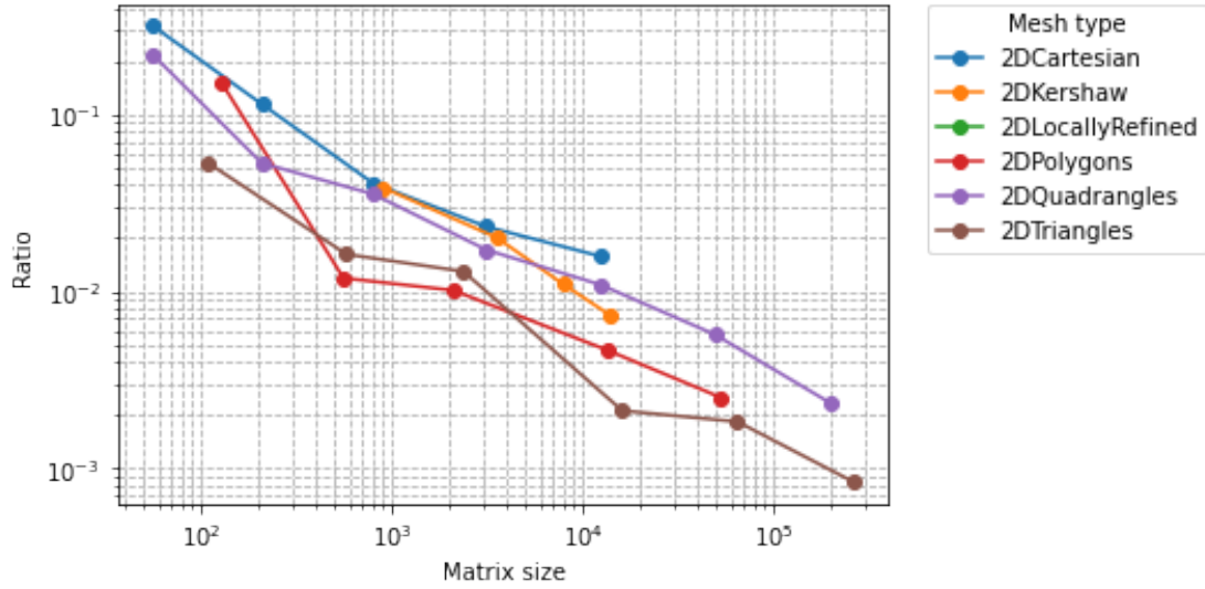
Residual / Error ratio vs. Matrix Size for Each Mesh Type in "2D" Type List
