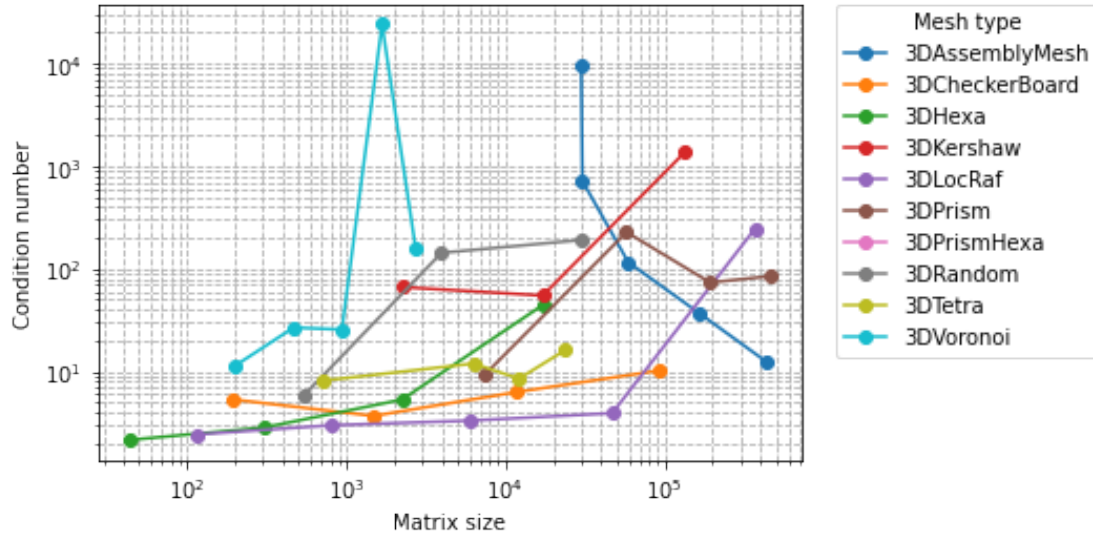
Condition Number vs. Matrix Size for Each Mesh Type in "3D" Type List
