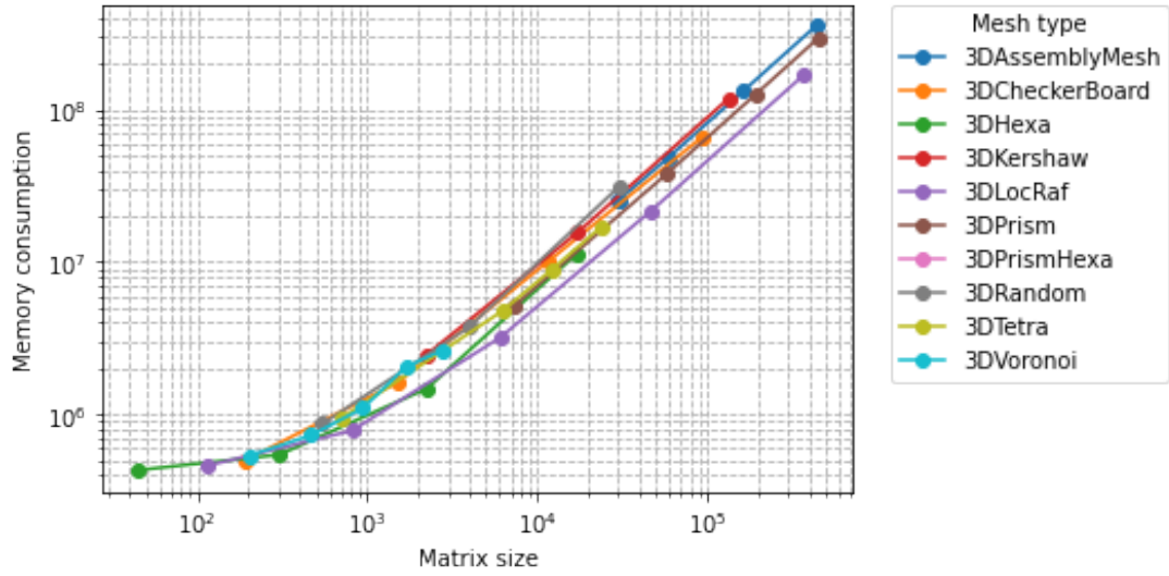
Memory Consumption vs. Matrix Size for Each Mesh Type in "3D" Type List
