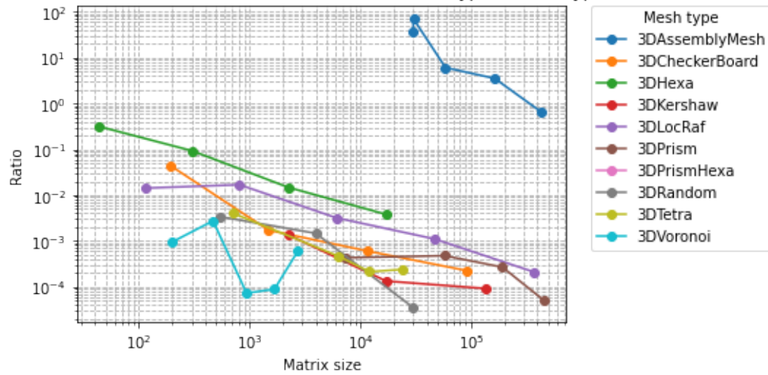
Residual / Error ratio vs. Matrix Size for Each Mesh Type in "3D" Type List
