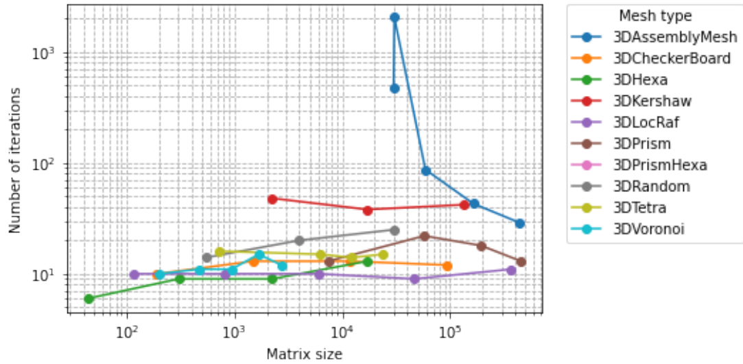
Number of iterations vs. Matrix Size for Each Mesh Type in "3D" Type List
