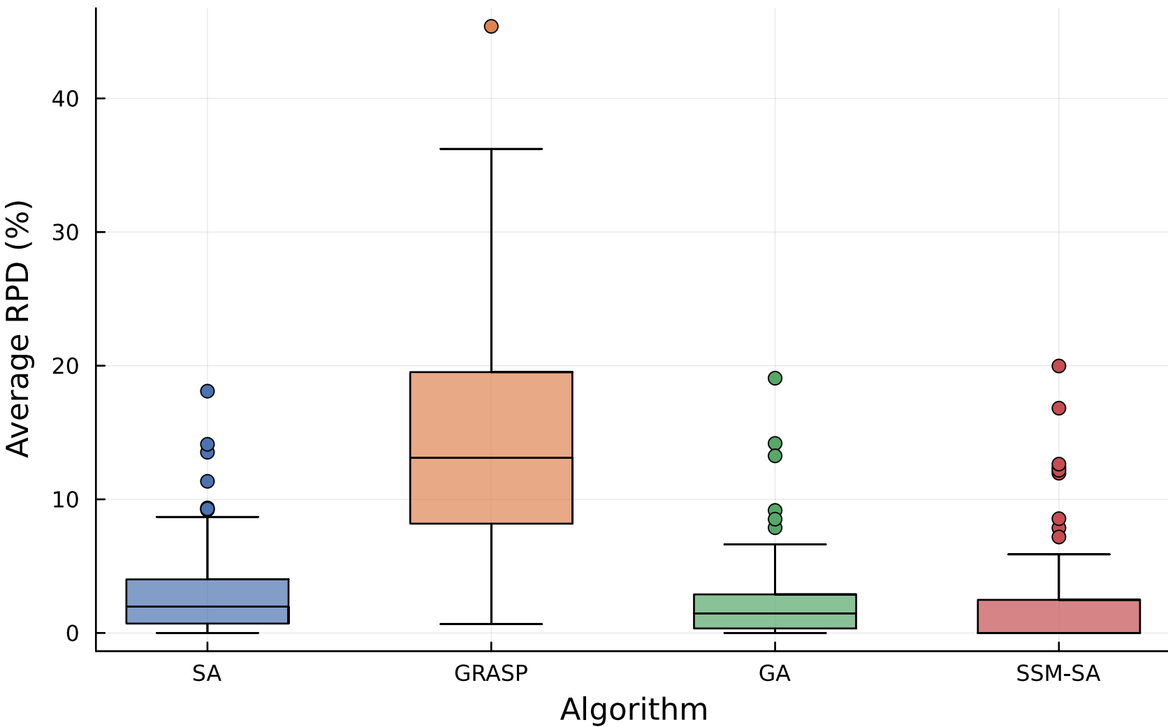
Distribution of per-instance average RPD
