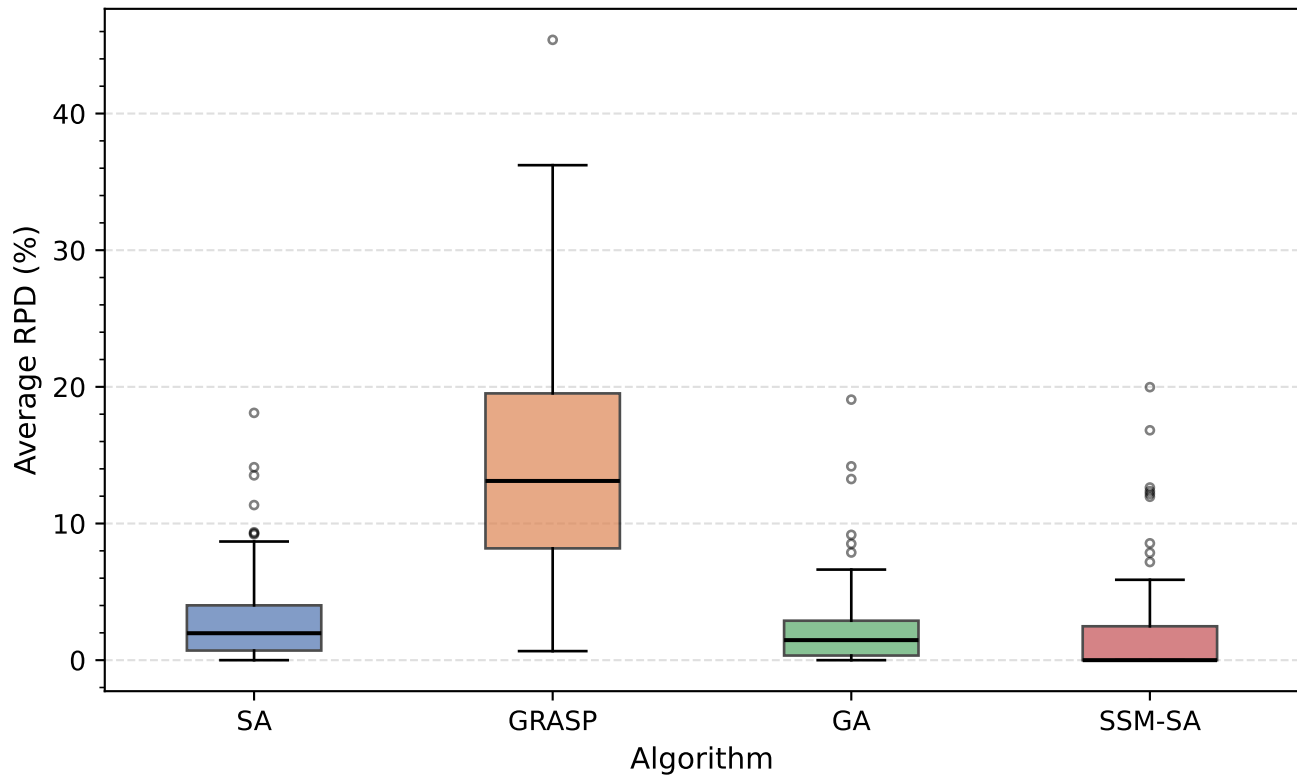
Distribution of per-instance average RPD
