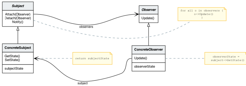
Figure 1: General Observer Design Pattern UML Diagram
