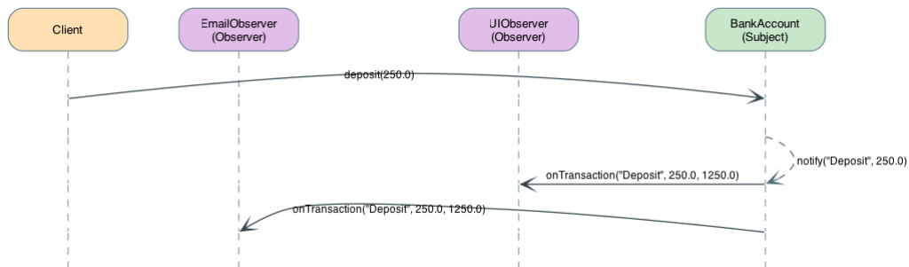
Figure 3: UML Sequence Diagram for Bank Account Notification Process
