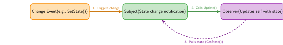
Figure 7: Sequential Process Flowchart of a Single Observer Notification
