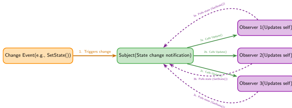
Figure 8: Sequential Process Flowchart with Multiple Observers (Pull Model)
