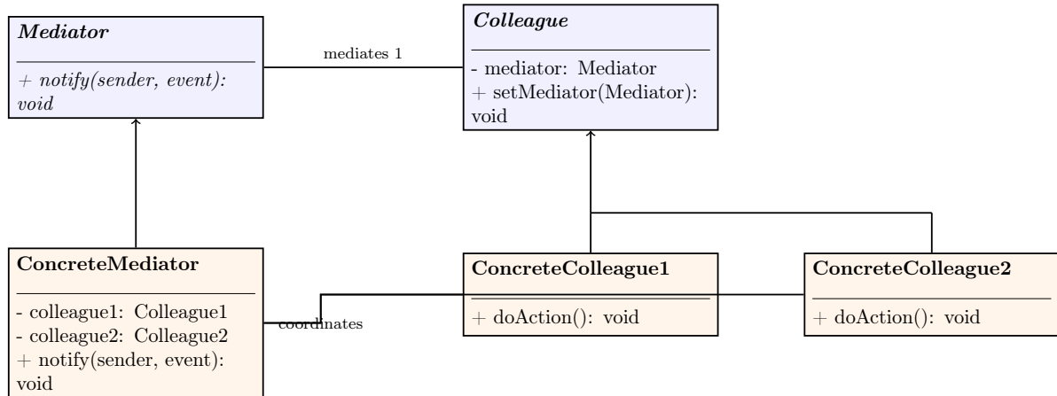
Figure 3: General GoF Mediator Pattern UML Structure
