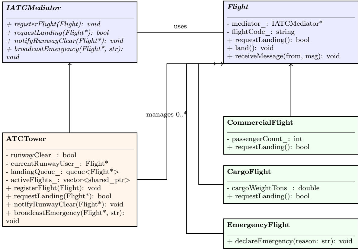
Figure 4: Airport Air Traffic Control Mediator Class Hierarchy
