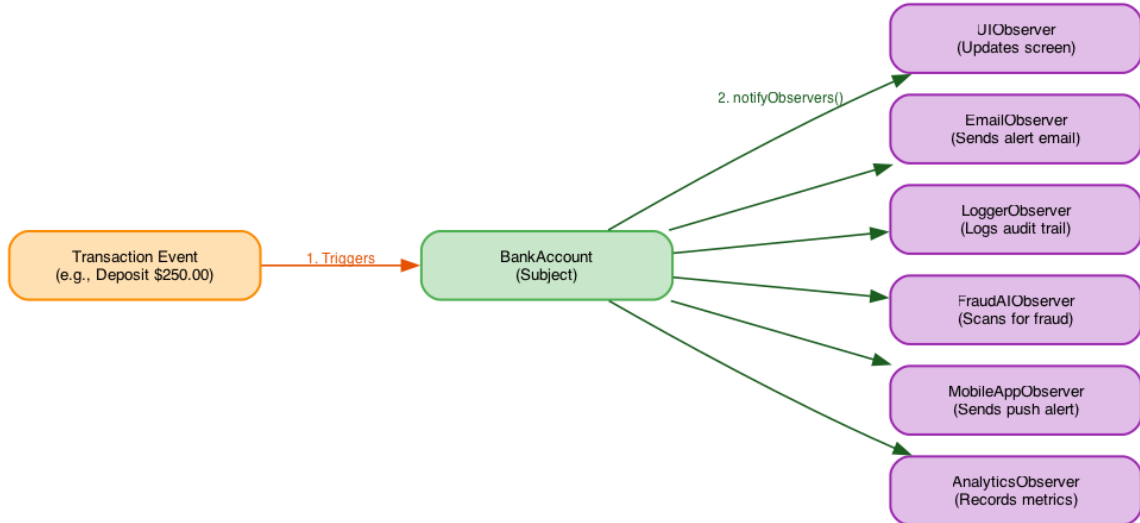
Figure 11: Process Flowchart for Bank Account Notification System (Push Model)
