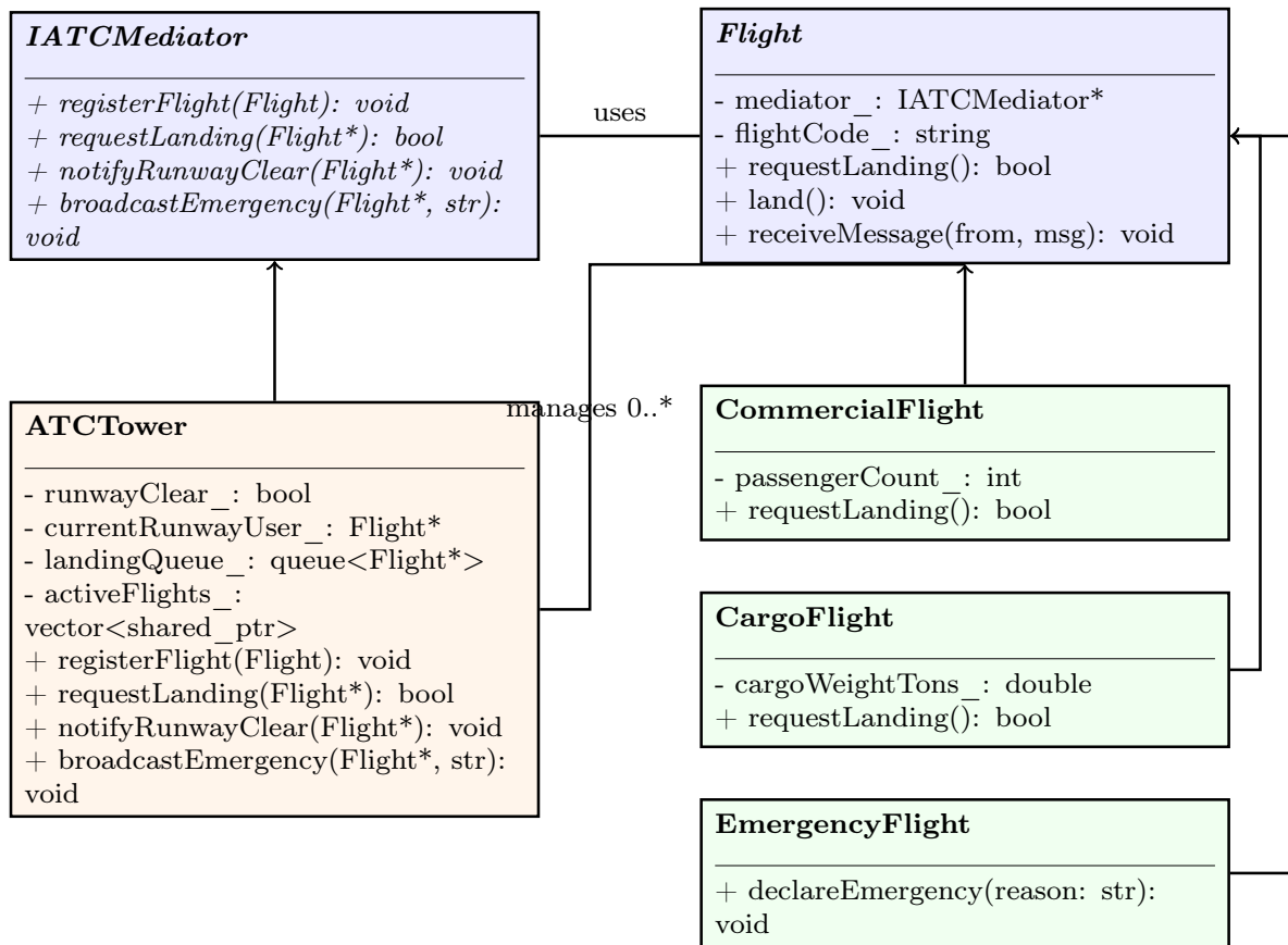
Figure 4: Airport Air Traffic Control Mediator Class Hierarchy
